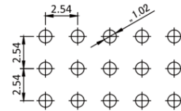
Recommended PCB Layout (PCB TOLERANCE ±0.05)
